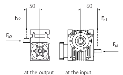
Bearing forces
