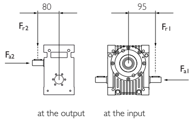
Bearing forces
