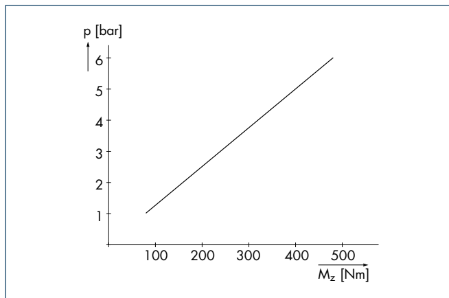
Type of load: Torsional ( M_z )
