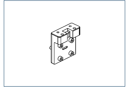
Mounting block SWM-TSS-3306 ID 0302582
