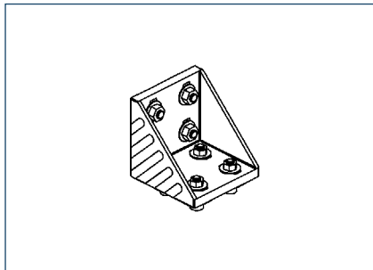
Stand bracket SWM-TSS-1030 ID 0302581
