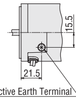
Detail Drawing of Protective Earth Terminal
