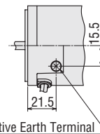
Detail Drawing of Protective Earth Terminal
