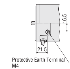
Detail Drawing of Protective Earth Terminal
