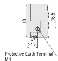
Detail Drawing of Protective Earth Terminal
