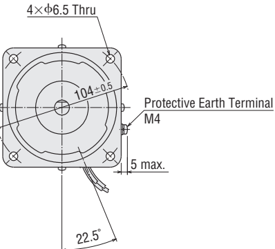
Detail Drawing of Protective Earth Terminal
