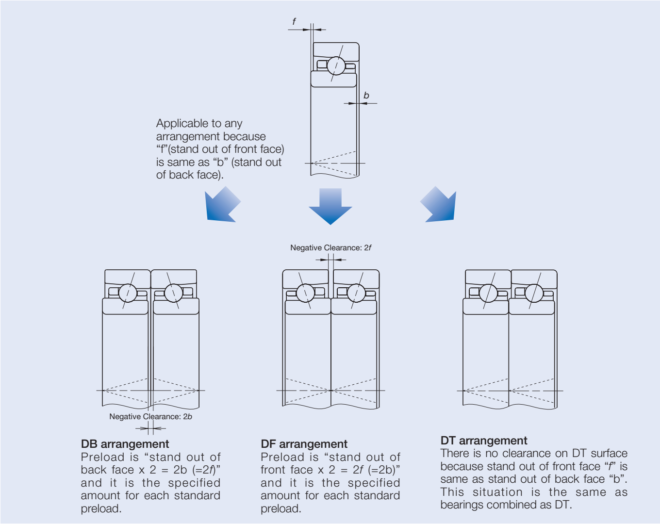
Fig. 3.7 Universal Combination
