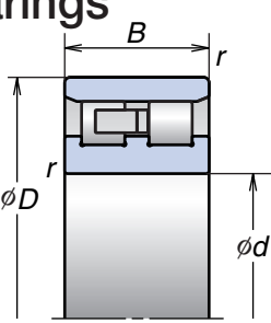
*NN39 Cylindrical Bore
