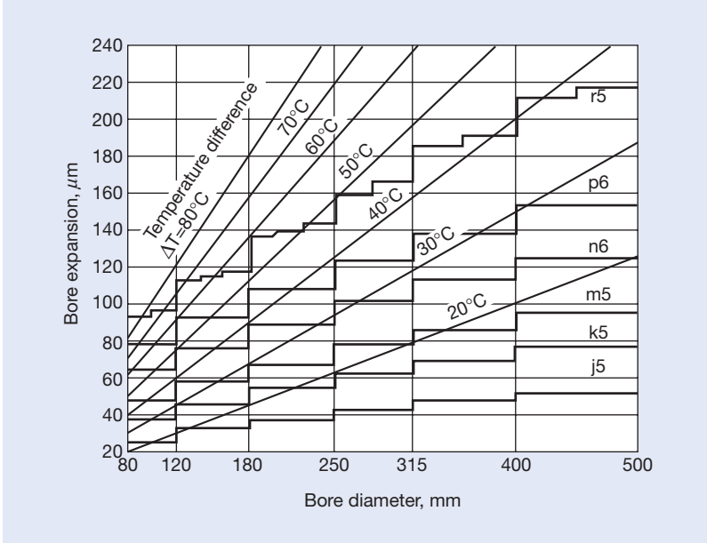
Fig. 1.2 Temperature and Thermal Expansion of Inner Ring
