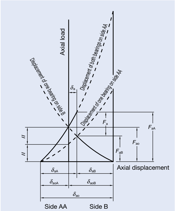
Fig. 4.6 Preloaded Axial Displacement of DBD Arrangement
