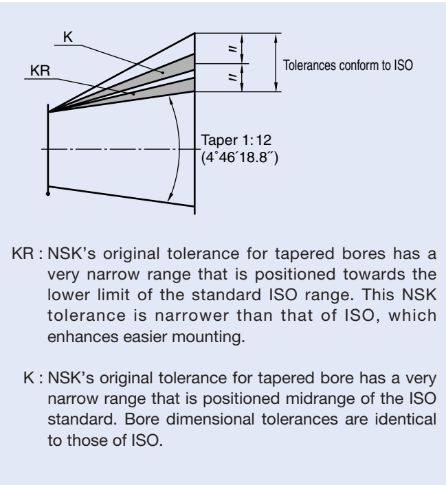
Fig. 7.2 Tolerances
