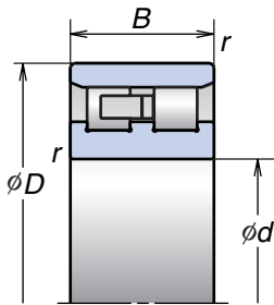
*Cylindrical Bore
