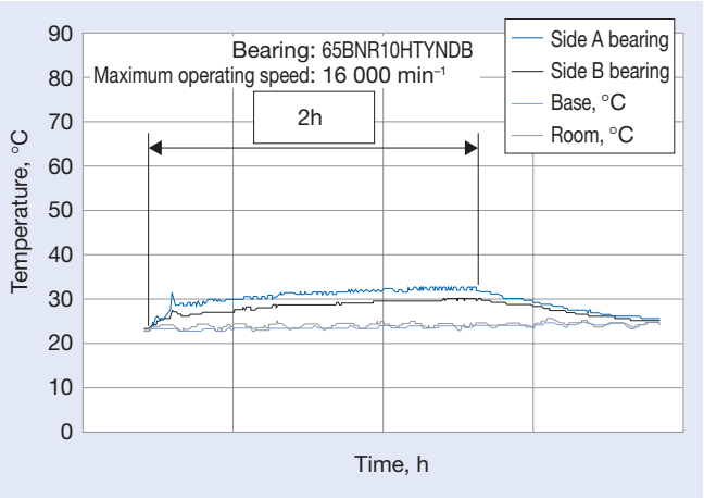
Fig. 3.4 One Cycle for Intermittent Running-in Procedure
