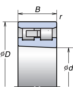
NN39 Tapered Bore
