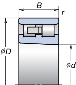
Tapered Bore
