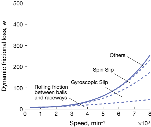
Calculated result of heat generation
