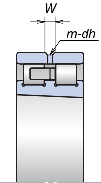
Lubrication Holes Dimensions (E44 Specification) Unit: mm
