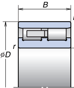
*NN49 Cylindrical Bore
