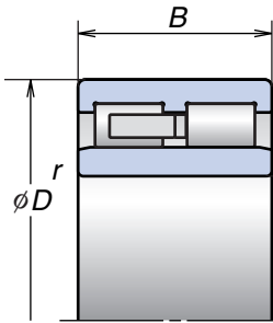
*NNU49 Cylindrical Bore
