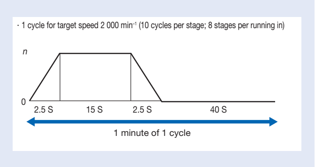
Fig. 3.4 One Cycle for Intermittent Running-in Procedure
