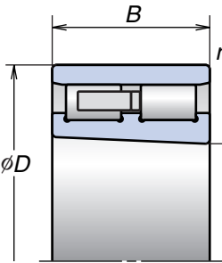
NN49 Tapered Bore
