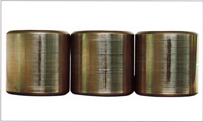
Photo 7-12-4 Part: Rollers of a cylindrical roller bearing Symptom: False brinelling occurs on rolling surface Cause: Vibration from an external source while stationary
