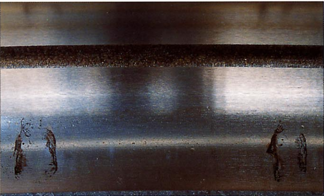
Photo 7-16-2 Part: Outer ring of a slewing ring Symptom: Rust on raceway surface at ball pitch Cause: Moisture condensation during stationary periods
