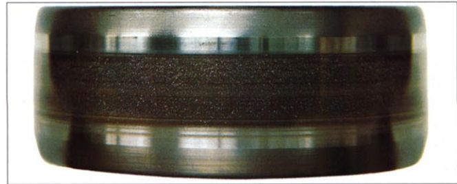
Photo 7-15-3 Part: Inner ring of a cylindrical roller bearing Symptom: Belt pattern of electrical corrosion accompanied by pits on the raceway surface
