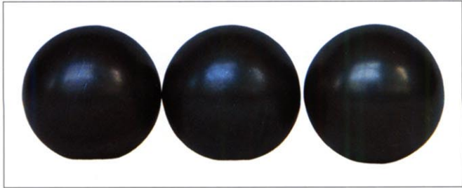
Photo 7-15-4 Part: Balls of a groove ball bearing Symptom: Electrical corrosion has a dark color that covers the entire ball surface
