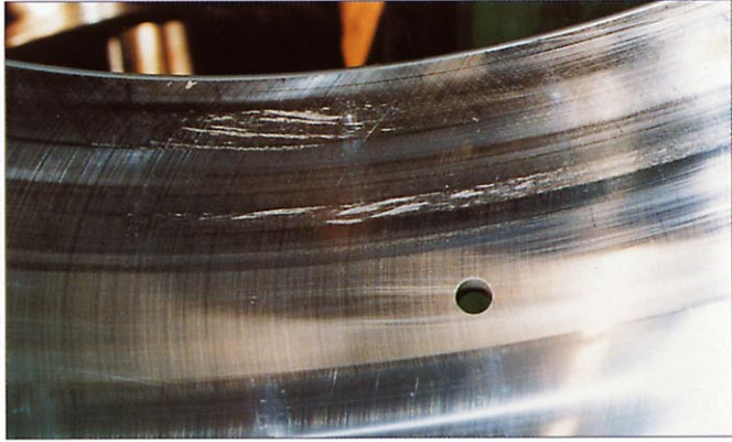
Photo 7-4-6 Part: Outer ring of Photo 7-4-5 Symptom: Partial smearing occurs circumferentially on raceway surface Cause: Poor lubrication
