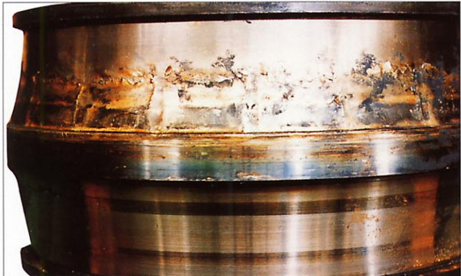
Photo 7-14-1 Part: Inner ring of a spherical roller bearing Symptom: Raceway is discolored and melted. Worn particles from the cage were rolled and attached to the raceway Cause: Insufficient lubrication
