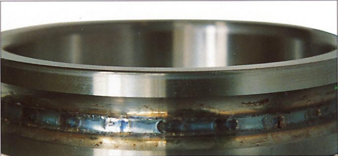
Photo 7-14-3 Part: Inner ring of an angular contact ball bearing Symptom: Raceway discoloration, melting occurs at ball pitch intervals Cause: Excessive preload
