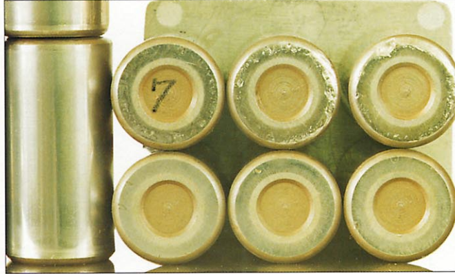
Photo 7-3-4 Part: Rollers of a double-row cylindrical roller bearing Symptom: Scoring on the roller end face Cause: Poor lubrication and excessive axial load
